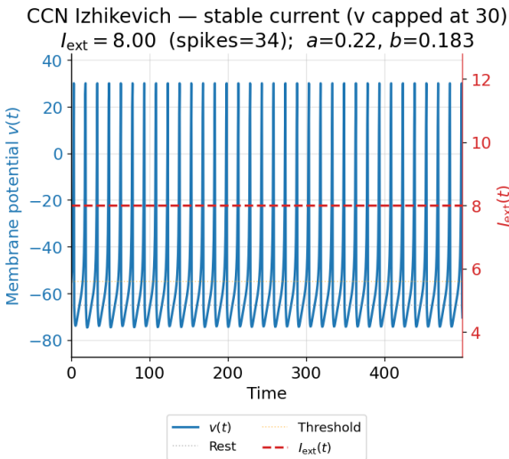
Fig. 6: Resulting spike train.
