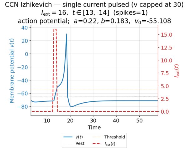
Fig. 12: Exactly one action potential occurred in spite of the height of the spike.
