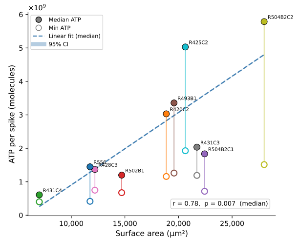
Fig. 2. Relationship between surface area and ATP consumption per morphology.
