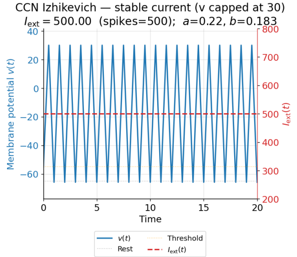
Fig. 8: Resulting spike train that no longer accommodates the absolute refractory period, as there is a spike occurring every unit of time due to the hard reset of the Izhikevich model.
