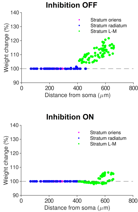
Fig. 4: Electrical theta-burst stimulation produces LTP in distal tuft when inhibition disabled. Top: Inhibition off. Bottom: Inhibition on.
