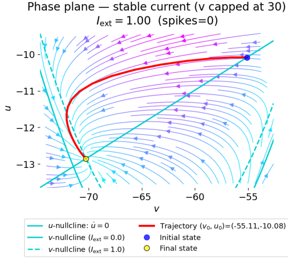
Fig. 1: Stable external current of height I_{ext} = 1.0 . Only a small oscillation happened, as the external current was too low to produce an action potential.
