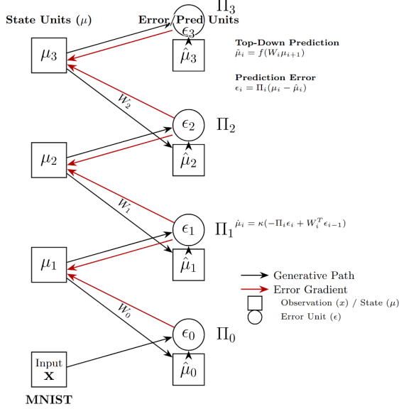
Fig. 1: Hybrid predictive coding architecture with precision matrices. Based on Tschshantz et al. (2023).
