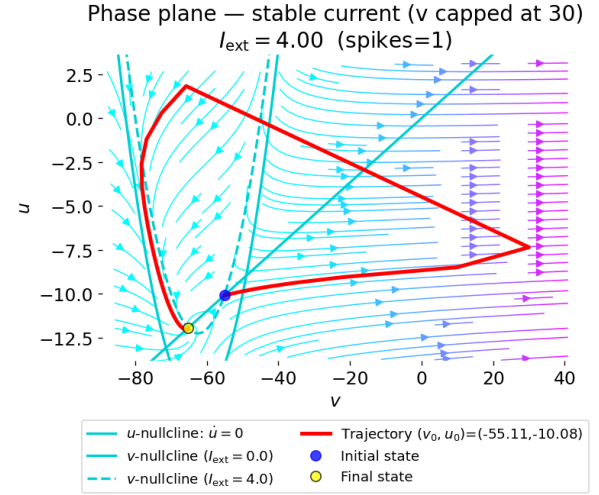
Fig. 3: Stable external current of height I_{ext} = 4.0 . Exactly one action potential occurred, even though the current was introduced permanently.
