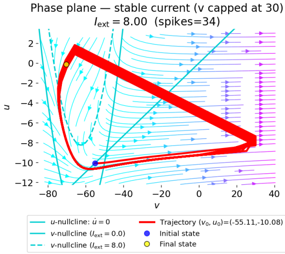
Fig. 5: A spike train occurs when I_{ext} = 8.0 , which can be seen by repetitive expeditions of the system through the phase plane. 34 spikes occur over a period of 500 units of time.
