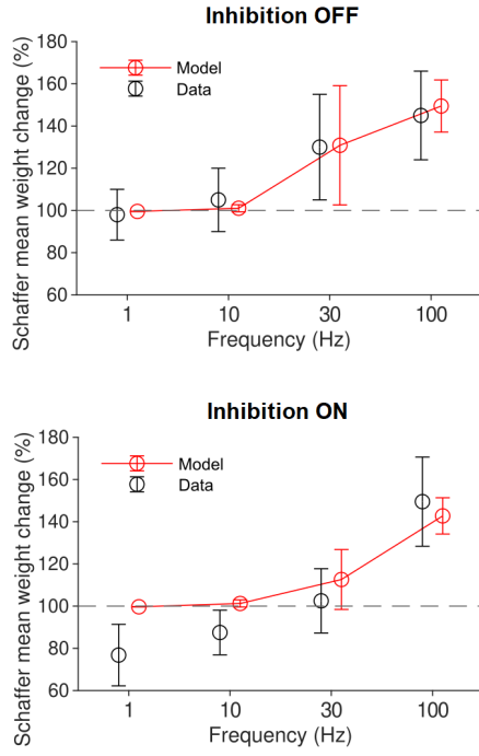
Fig. 2: Model reproduces electrical stimulation data from Ikegaya et al. for most frequencies. Top: Frequency dependence with inhibition off. Bottom: Frequency dependence with inhibition on.
