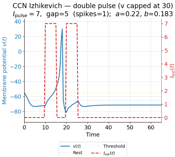
Fig. 14: Resulting voltage curve of one spike and one small oscillation.
