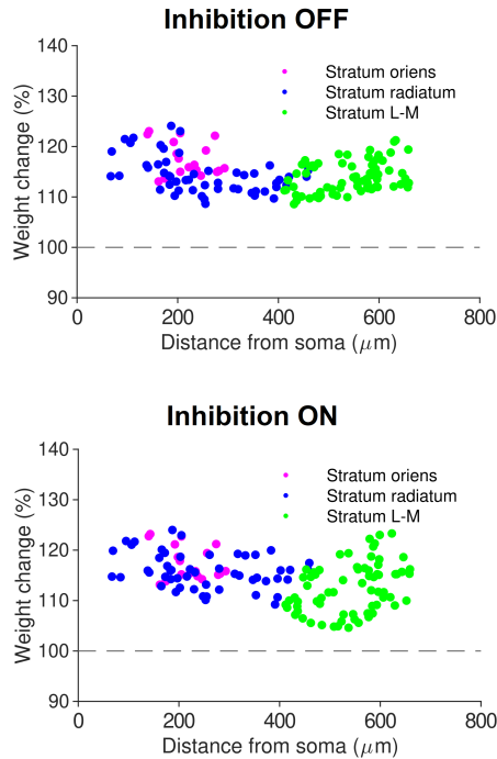
Fig. 5: Magnetic theta-burst stimulation produces LTP all over the cell both with and without inhibition. Top: Inhibition off. Bottom: Inhibition on.
