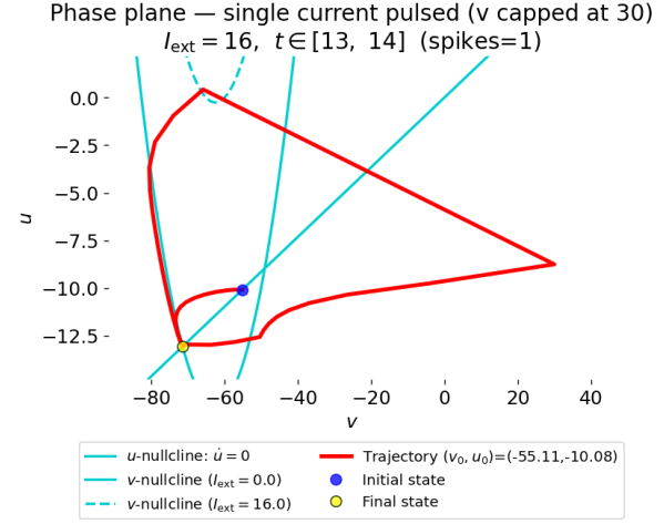
Fig. 11: As the spike was introduced only for a short unit of time, it did not result in a spike train, as it would have if it were introduced permanently.
