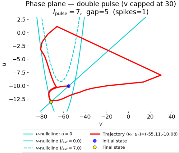
Fig. 13: Due to the absolute refractory period, no second spike occurred.
