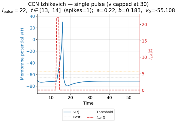
Fig. 10: The resulting action potential from a single pulse of height I = 22 , at time [13,14].
