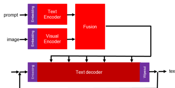
Fig. 6. Schema of transformer-based OCR
