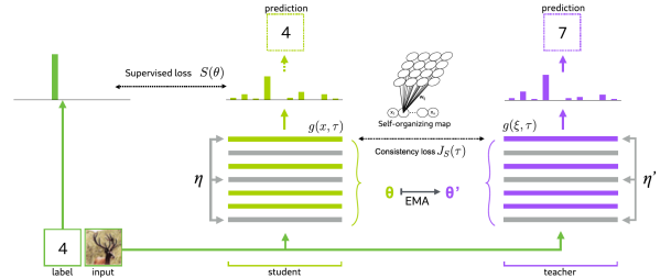
Fig. 2: Illustration of MT-SOM model, figure taken from Samporová (2024)
