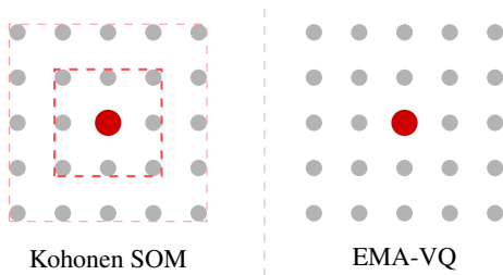
Fig. 1: The Kohonen self-organizing map update with Gaussian neighborhood (left) reduces to the EMA-VQ codebook update under zero neighborhood width (right). The red node marks the best-matching unit; dashed rectangles indicate the neighborhood support. Inspired by (Irie et al., 2024).
