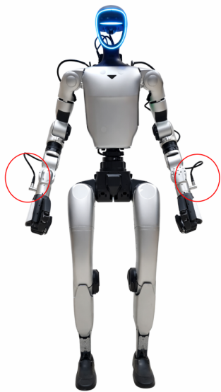
Fig. 1: Humanoid Unitree G1 EDU U6 with dexterous tactile hands RH56DFTP. Problematic external cable connection to hand containing power supply and control wires is marked by red ellipses.
