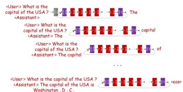
Fig. 1. Decoder-only transformer in the action
