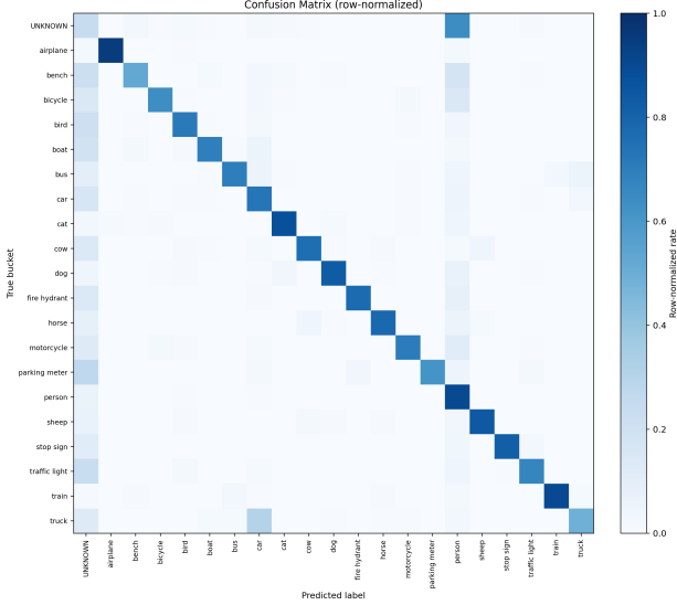
Fig. 1: Confusion matrix of MHN-based classification. The model shows strong diagonal structure for known classes, but a tendency to assign unknown samples to known categories.
