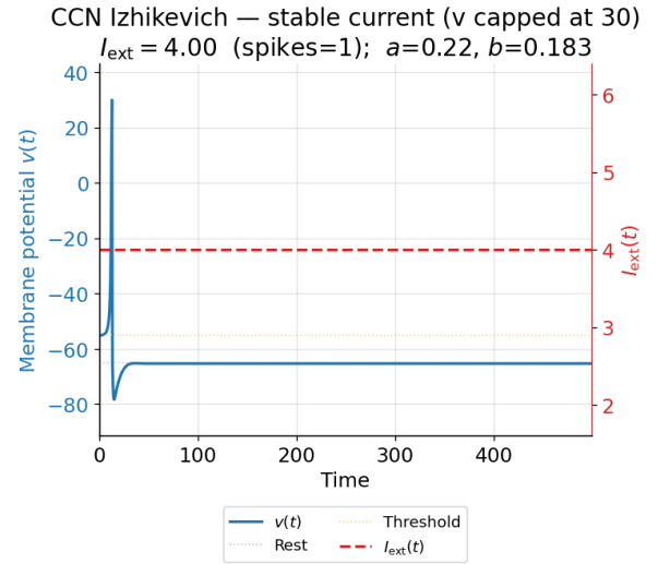
Fig. 4: The resulting singular action potential.
