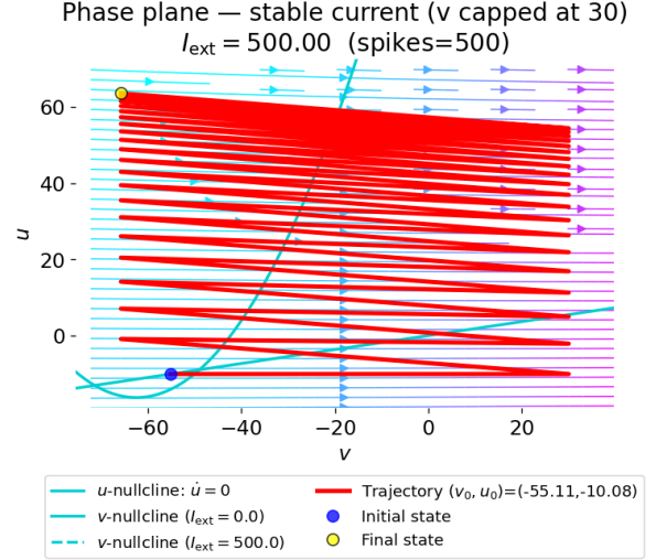
Fig. 7: When I_{ext} = 500.0 , the system is no longer able to sustain the absolute refractory period due to hard reset values. The time period used in the graph was shortened for better readability, but the simulation ran over 500 units of time, producing 500 spikes.
