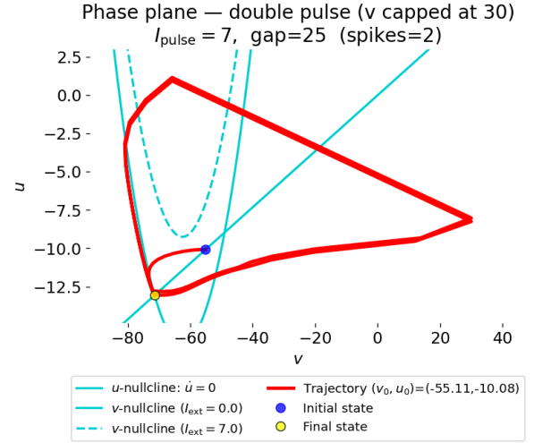
Fig. 15: As both the absolute and relative refractory periods had passed, the neuron was capable of producing two full spikes.
