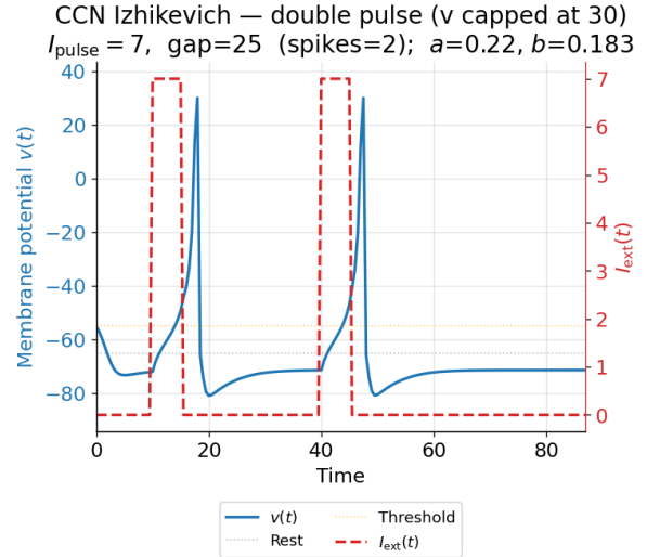
Fig. 16: Two fully pronounced spikes as a result of the two pulses with a large enough distance.
