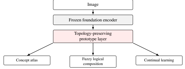
Fig. 4: The proposed pipeline. Images are passed through a frozen foundation encoder; the resulting features are routed through a topology-preserving prototype layer, a differentiable self-organizing map, whose grid serves as a shared substrate for the three downstream affordances.
