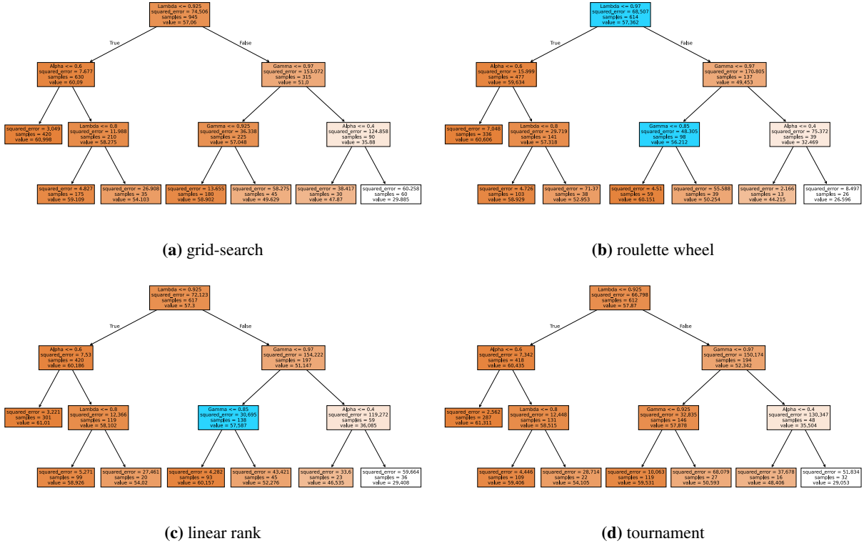
Fig. 2: Regression trees explaining the influence of hyperparameters on the AIQ of Q-learning in the coverage experiment. Differences in split tests between the grid-search and the genetic algorithm with roulette wheel, linear rank, and tournament selection modes are highlighted.
