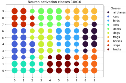
Fig. 3: CIFAR-10 MT-SOM neuron-activation grid, from (Samporová, 2024).
