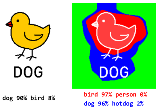
Fig. 8. An example of controversy named by CLIP and named partitioned by an agnostic algorithm FastNCut
