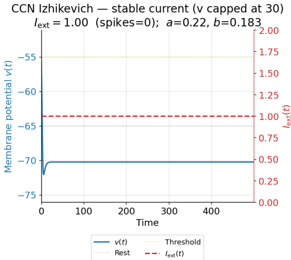
Fig. 2: No action potential occurred. The "ghost equilibrium" that was set up can be seen at time 0, as there is an initial displacement from the actual equilibrium.
