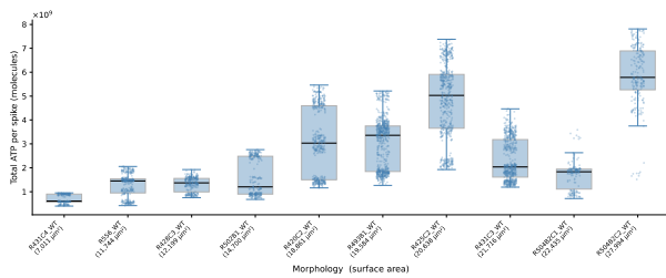
Fig. 1. Total ATP consumed per spike across 10 morphologies of different sizes, ordered by surface area.
