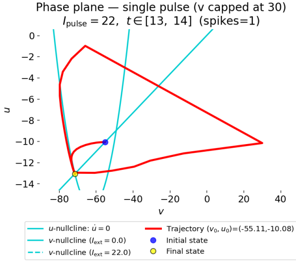
Fig. 9: Singular pulse at a time [13,14]. The pulse resulted in an action potential, as seen in a large enough dislocation of the system from the equilibrium point.
